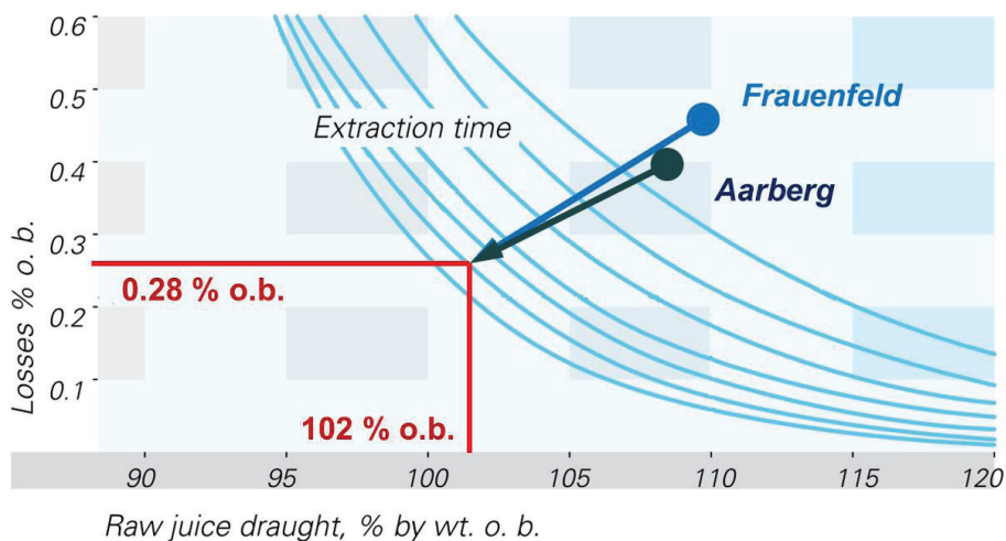
Fig. 4: Raw juice draft and sugar losses of the Frauenfeld and Aarberg sugar factories before and after modernisation of the extraction plant (campaign average)
